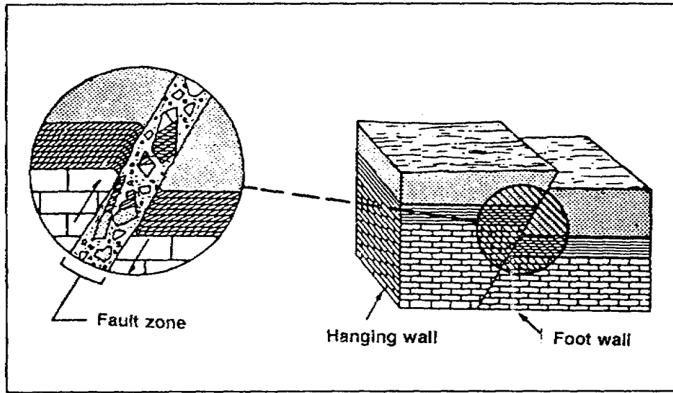
Figure 2-10. Reverse fault
